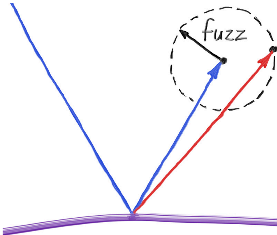
Figure 16: Generating fuzzed reflection rays
