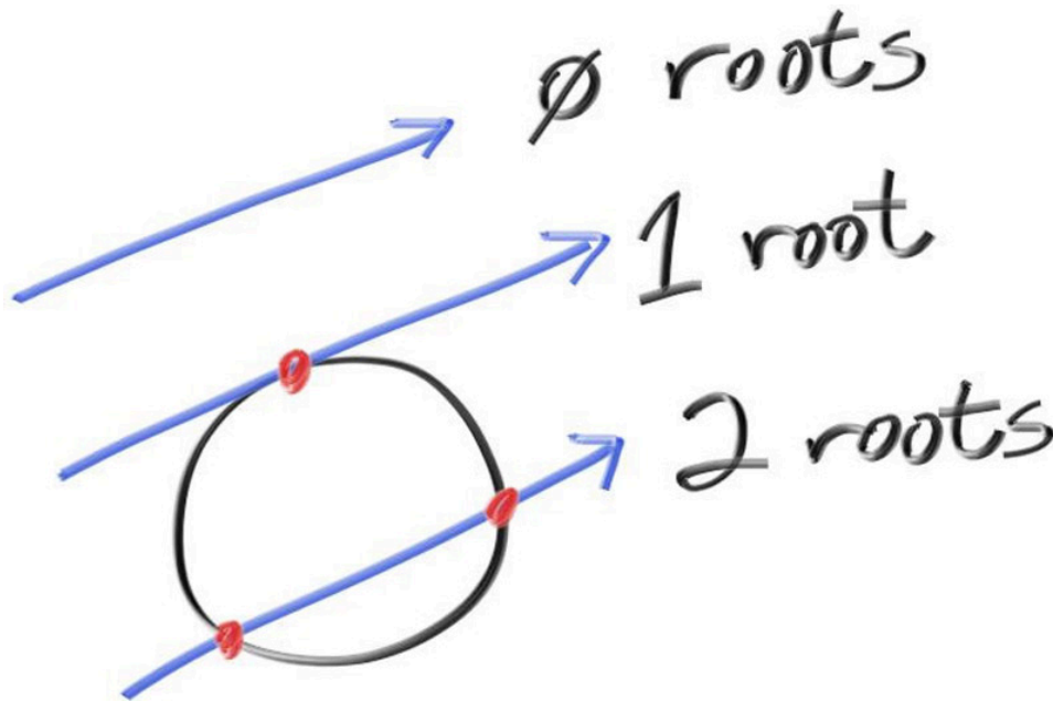
Figure 5: Ray-sphere intersection results
