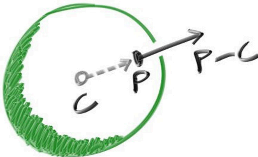
Figure 6: Sphere surface-normal geometry
